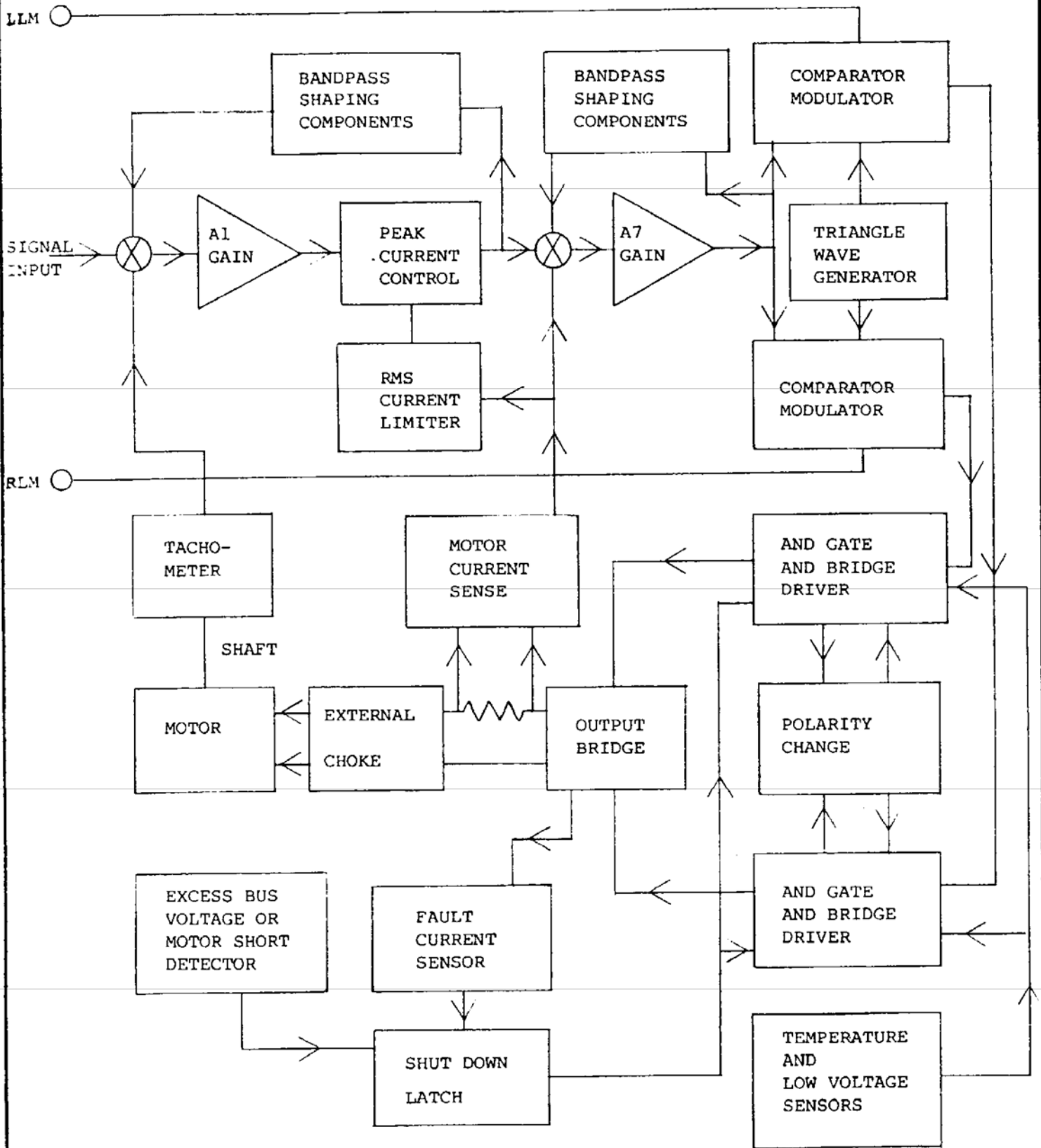
BLOCK DIAGRAM
