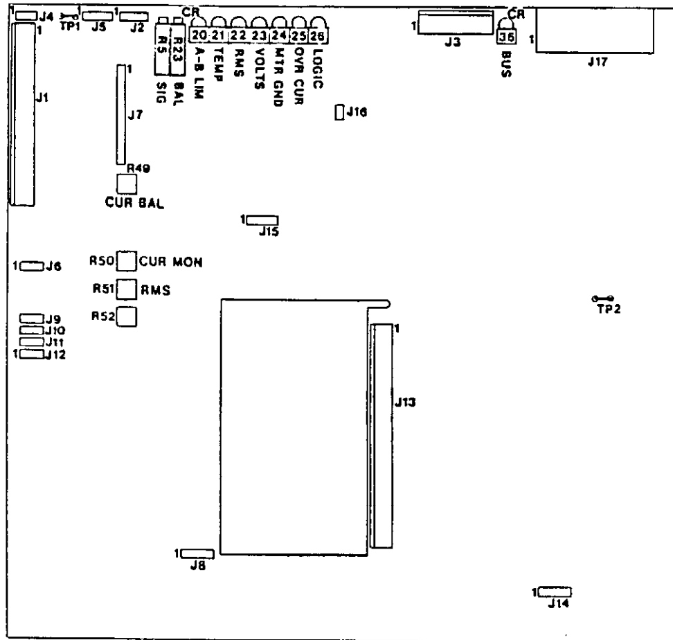
A722 SIMPLIFIED CONTROL BOARD LAYOUT
